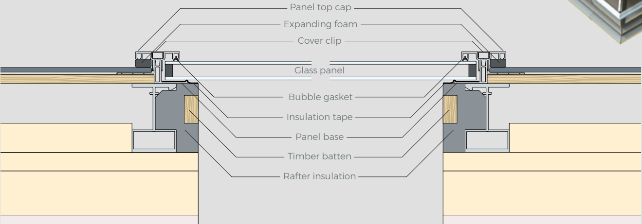
Guardian Solstice Rooflight System Detail
